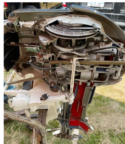
Rob Abbott's 1957 Johnson Javelin Cut-Away.
